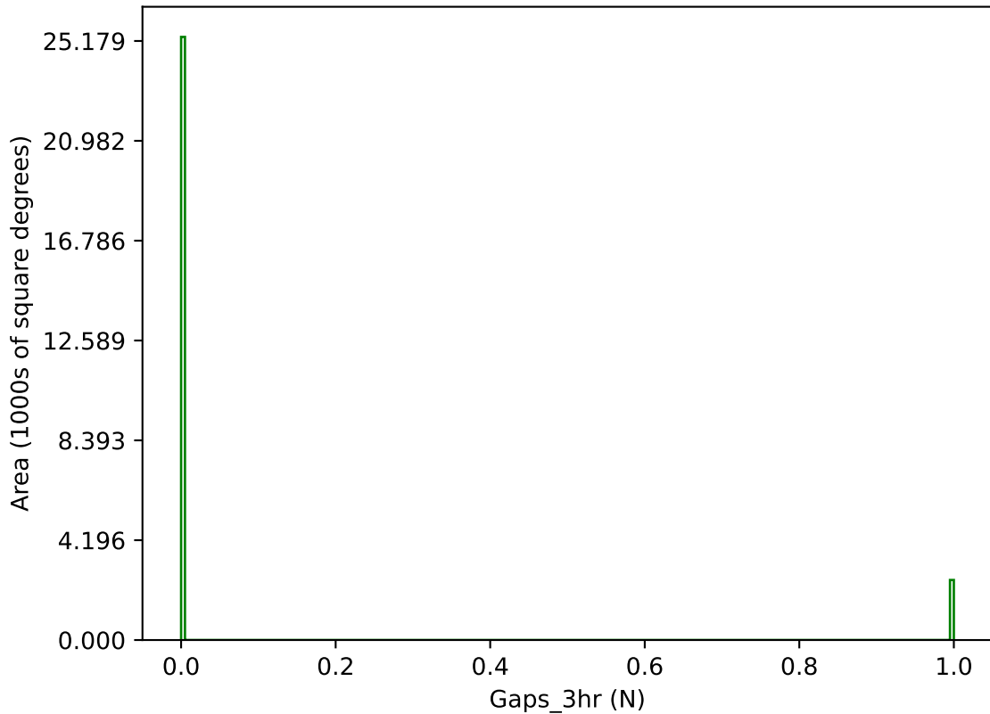
too_5_1v3.4_10yrs g band: Gaps_3hr
