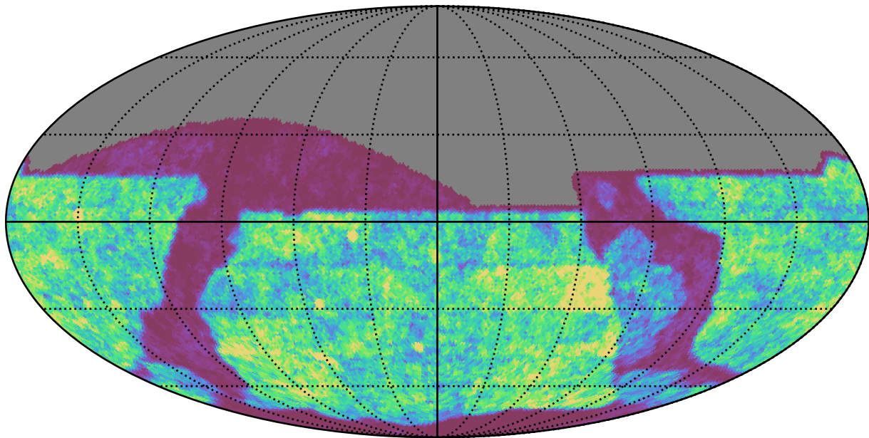
too_5_1v3.4_10yrs z band: Gaps_24hr
