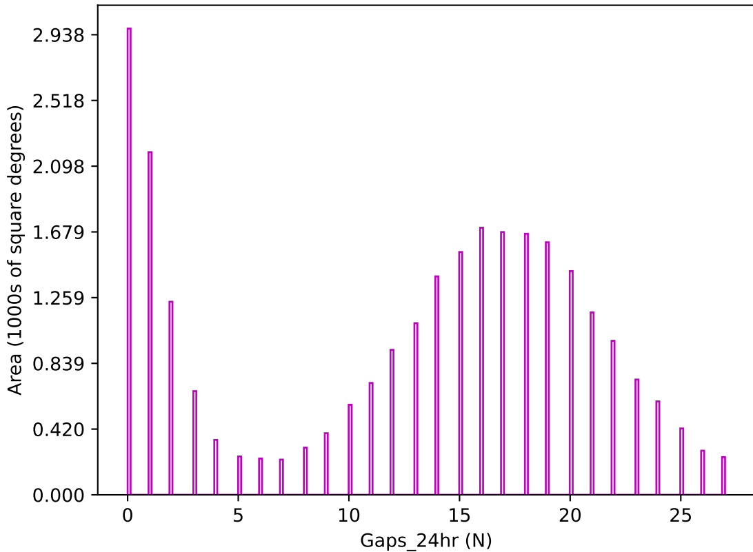
too_5_1v3.4_10yrs z band: Gaps_24hr
