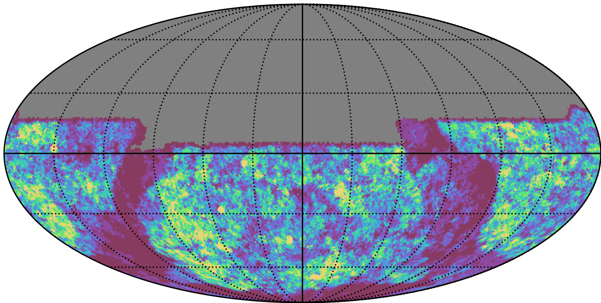
too_5_1v3.4_10yrs u band: Gaps_24hr
