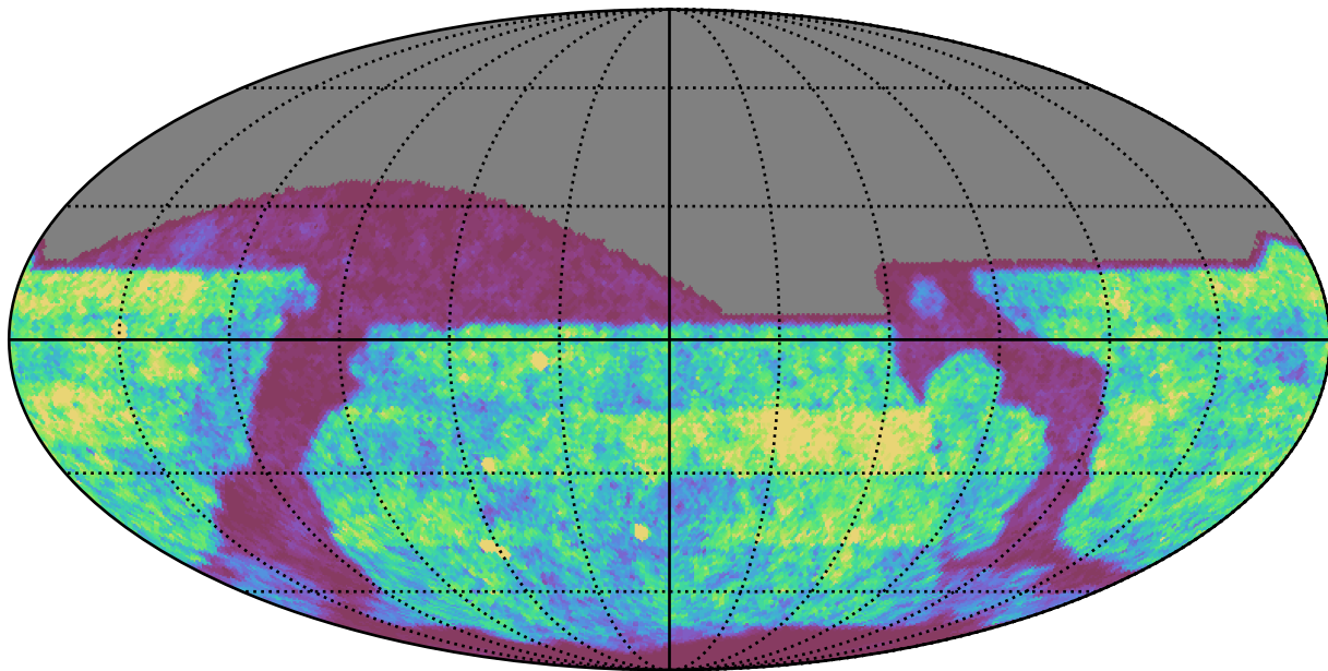
too_5_1v3.4_10yrs i band: Gaps_24hr
