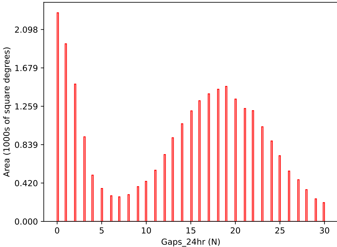
too_5_1v3.4_10yrs i band: Gaps_24hr
