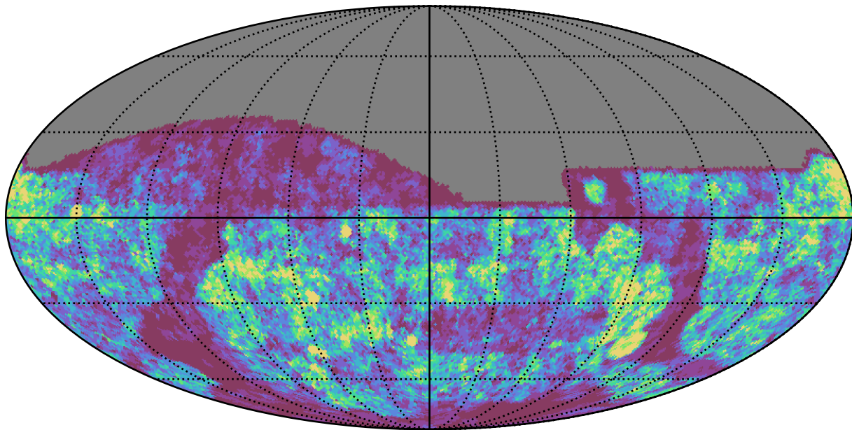
too_5_1v3.4_10yrs g band: Gaps_24hr
