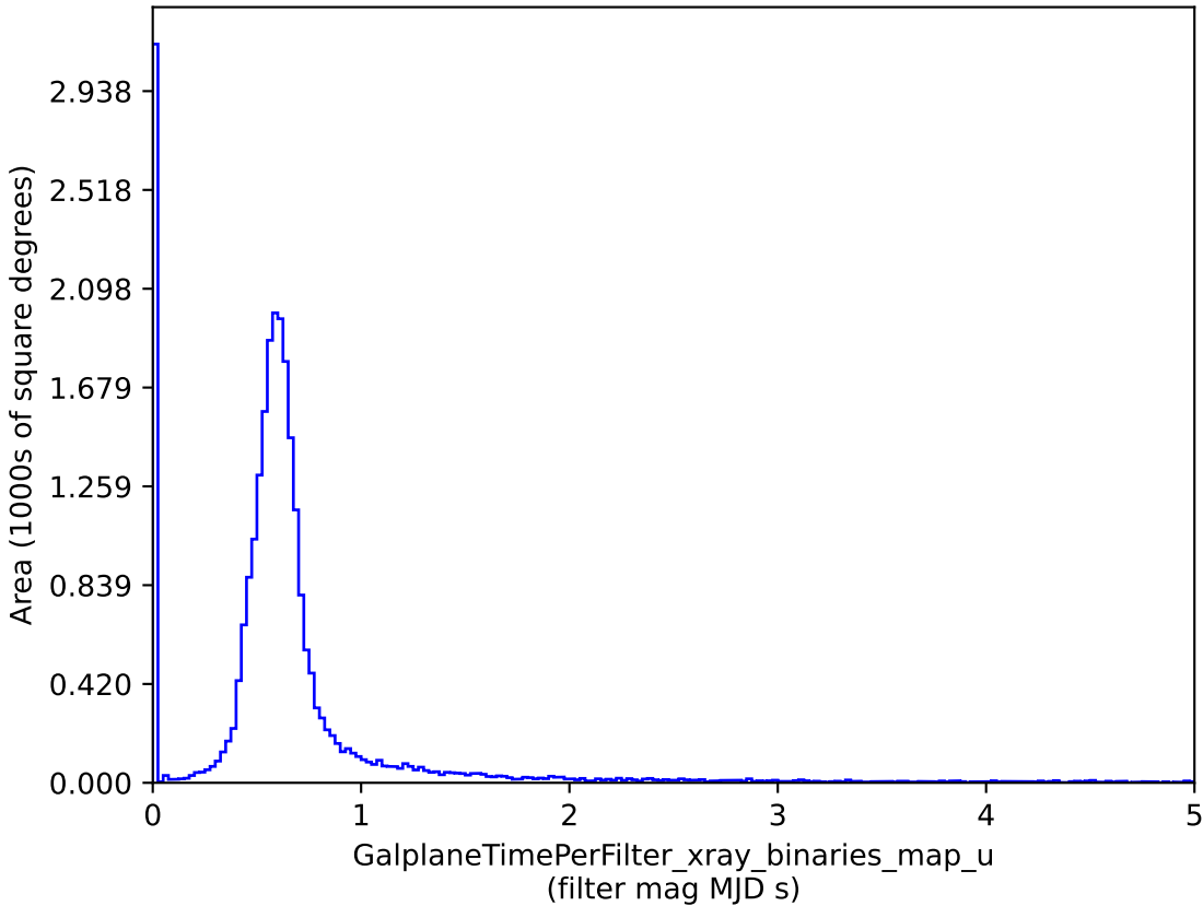
too_5_1v3.4_10yrs : GalplaneTimePerFilter_xray_binaries_map_u
