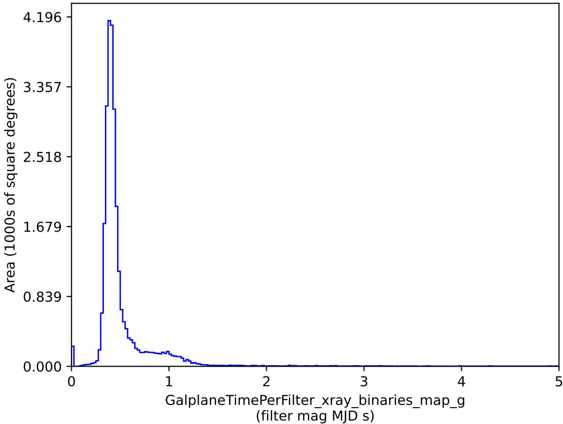
too_5_1v3.4_10yrs : GalplaneTimePerFilter_xray_binaries_map_g
