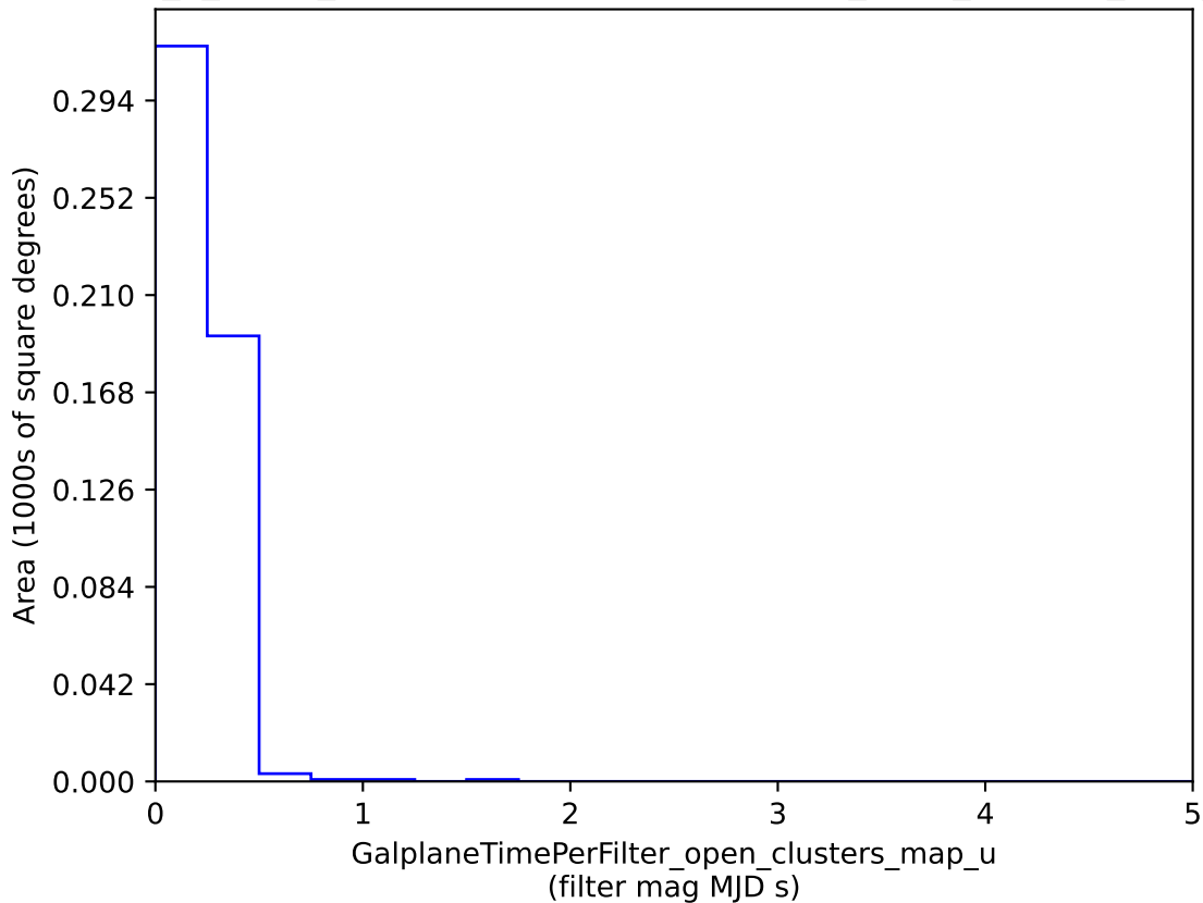
too_5_1v3.4_10yrs : GalplaneTimePerFilter_open_clusters_map_u
