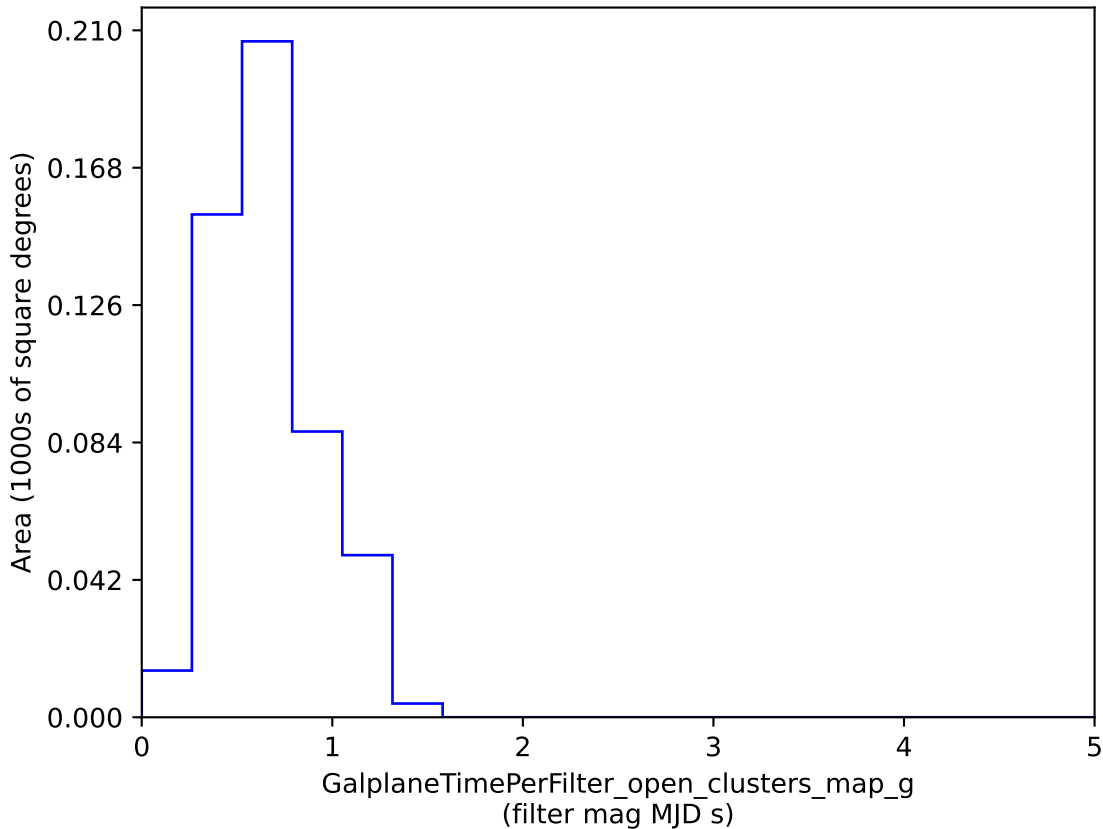
too_5_1v3.4_10yrs : GalplaneTimePerFilter_open_clusters_map_g
