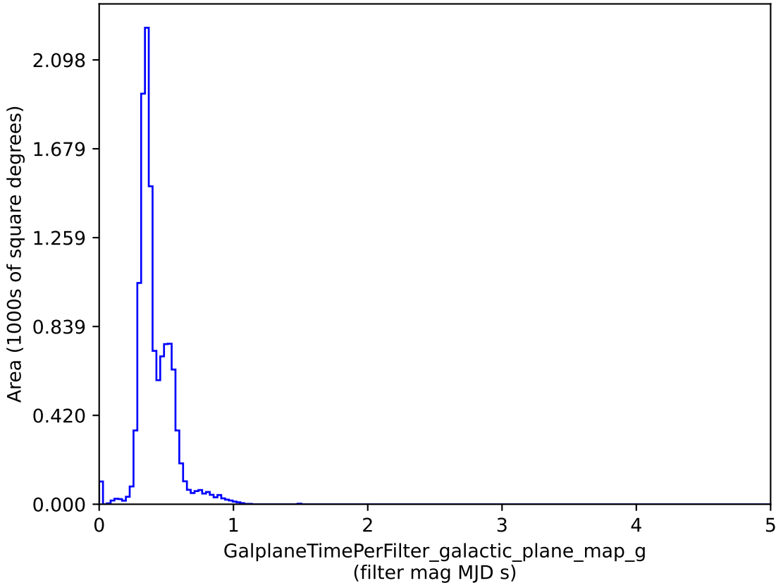
too_5_1v3.4_10yrs : GalplaneTimePerFilter_galactic_plane_map_g
