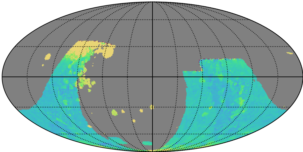
too_5_1v3.4_10yrs : GalplaneTimePerFilter_combined_map_z
