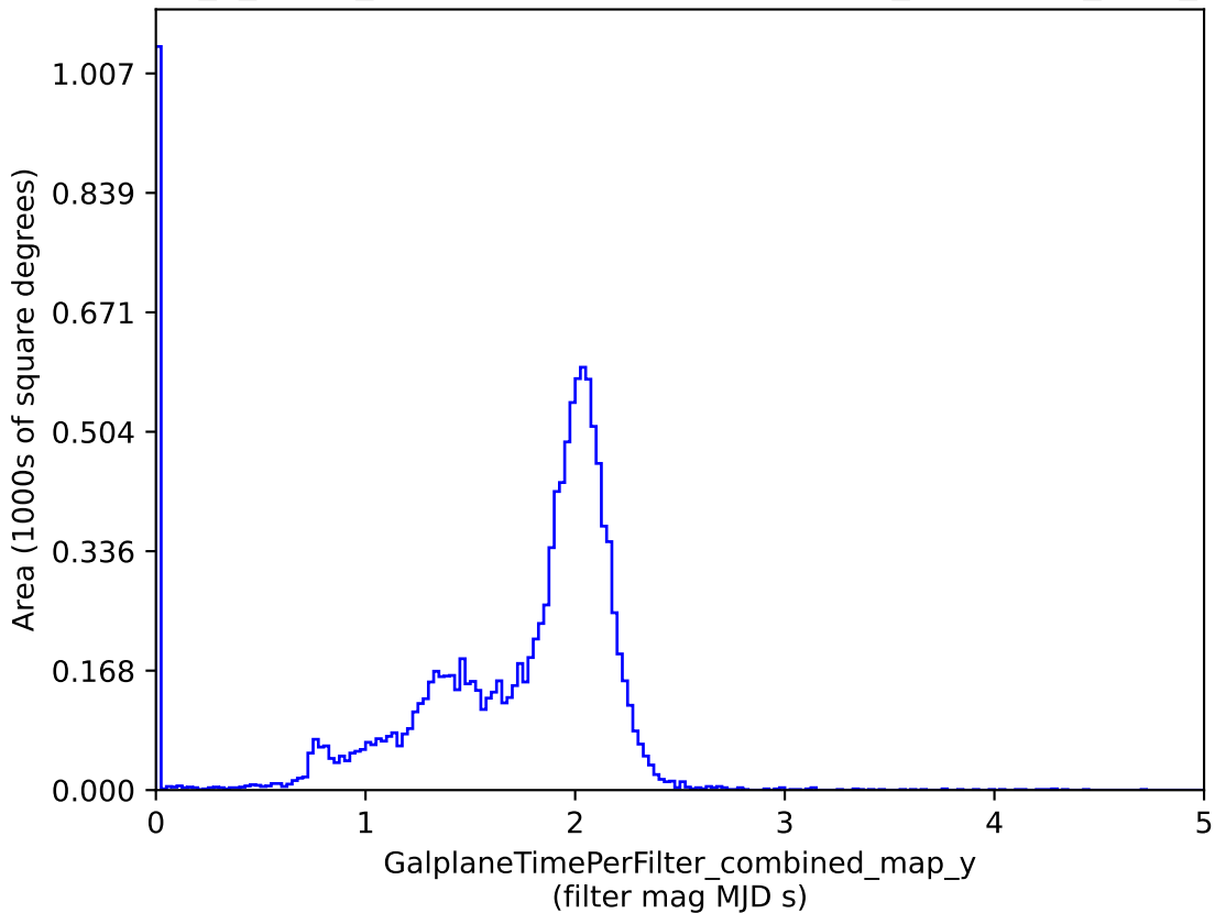
too_5_1v3.4_10yrs : GalplaneTimePerFilter_combined_map_y
