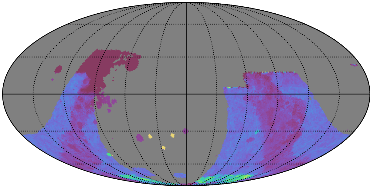
too_5_1v3.4_10yrs : GalplaneTimePerFilter_combined_map_u
