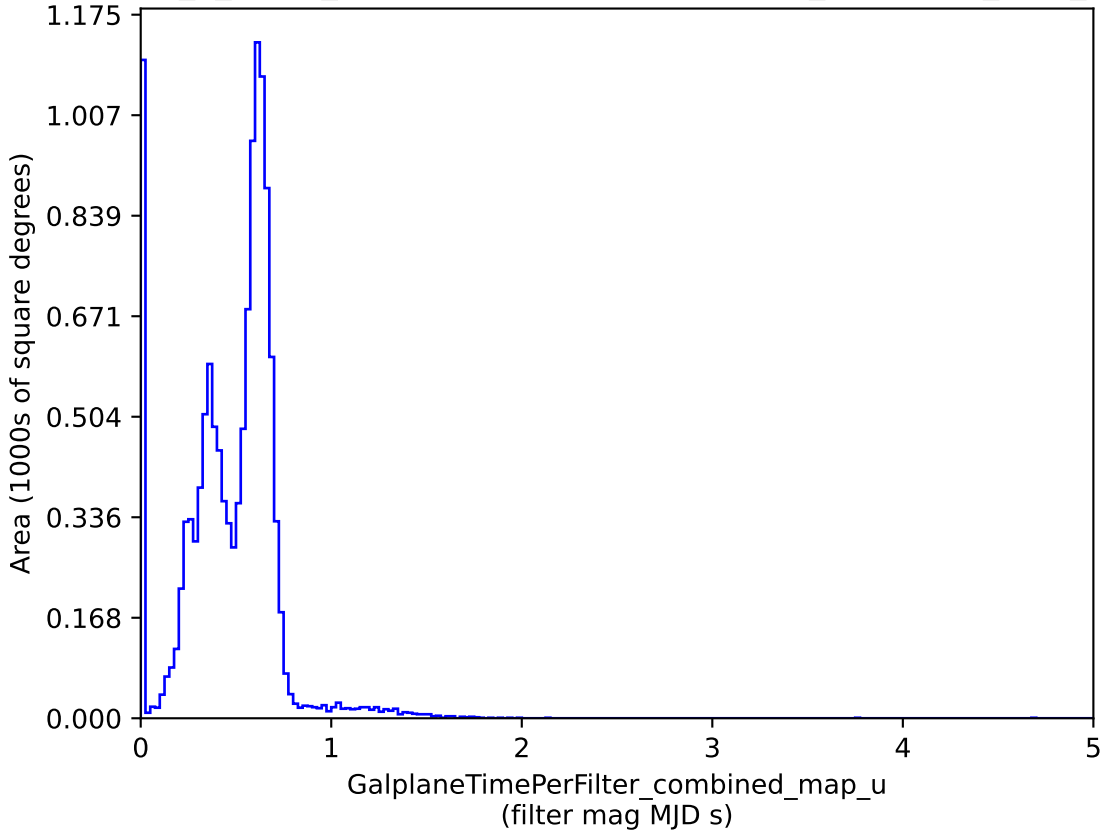
too_5_1v3.4_10yrs : GalplaneTimePerFilter_combined_map_u
