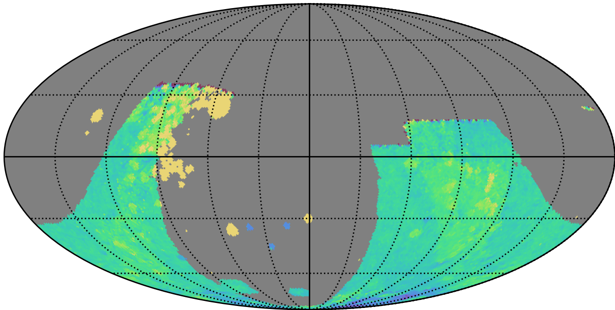
too_5_1v3.4_10yrs : GalplaneTimePerFilter_combined_map_i
