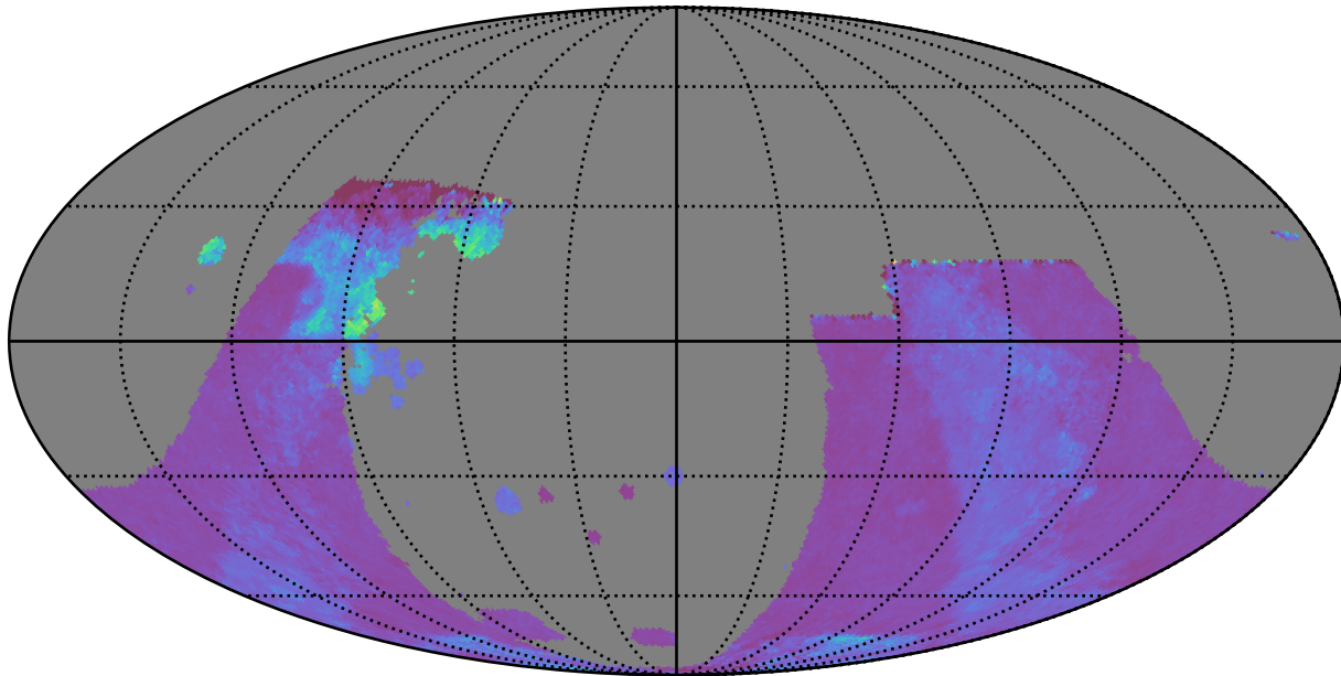
too_5_1v3.4_10yrs : GalplaneTimePerFilter_combined_map_g
