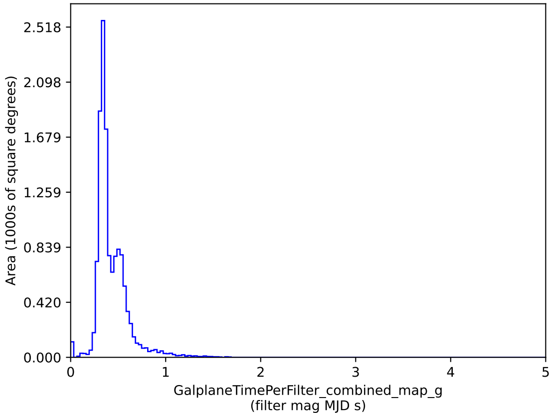
too_5_1v3.4_10yrs : GalplaneTimePerFilter_combined_map_g
