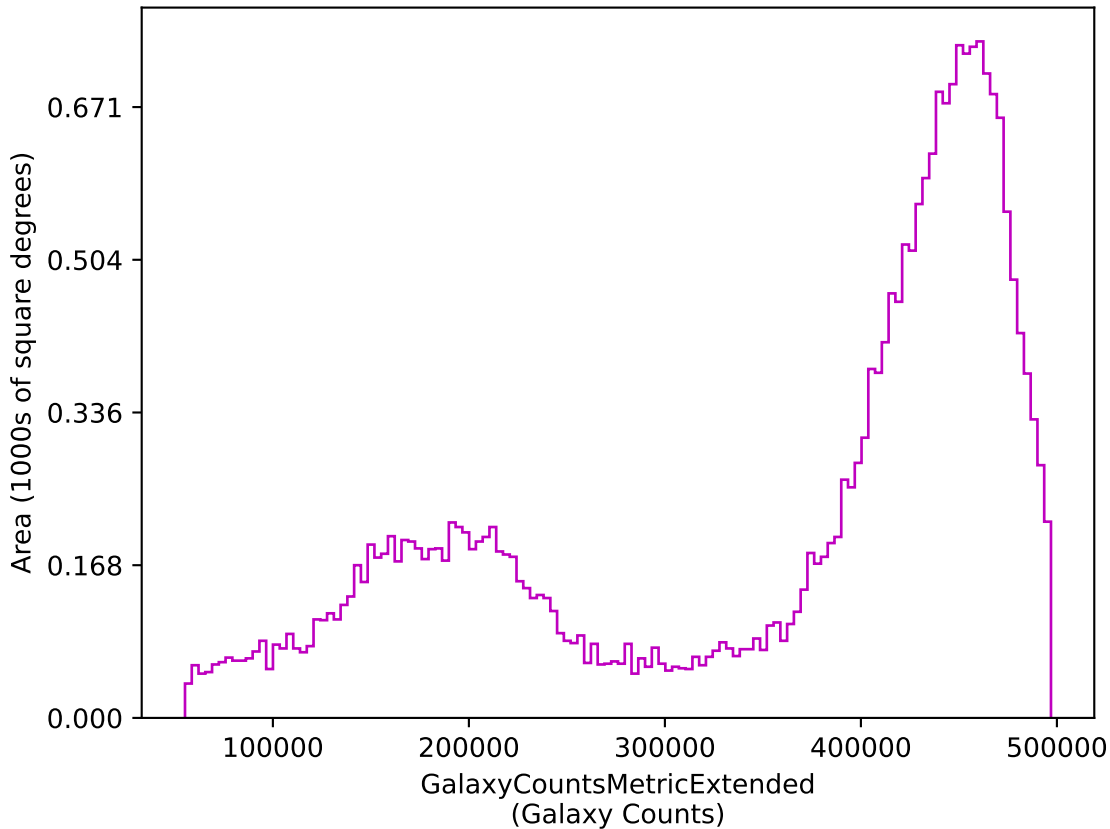
too_5_1v3.4_10yrs z: GalaxyCountsMetricExtended
