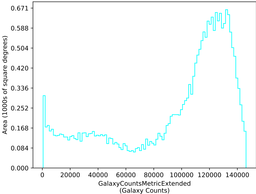
too_5_1v3.4_10yrs u: GalaxyCountsMetricExtended
