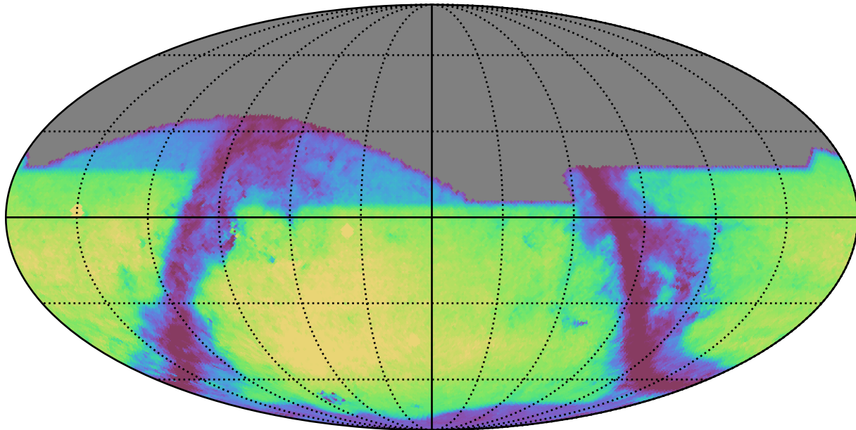
too_5_1v3.4_10yrs r: GalaxyCountsMetricExtended
