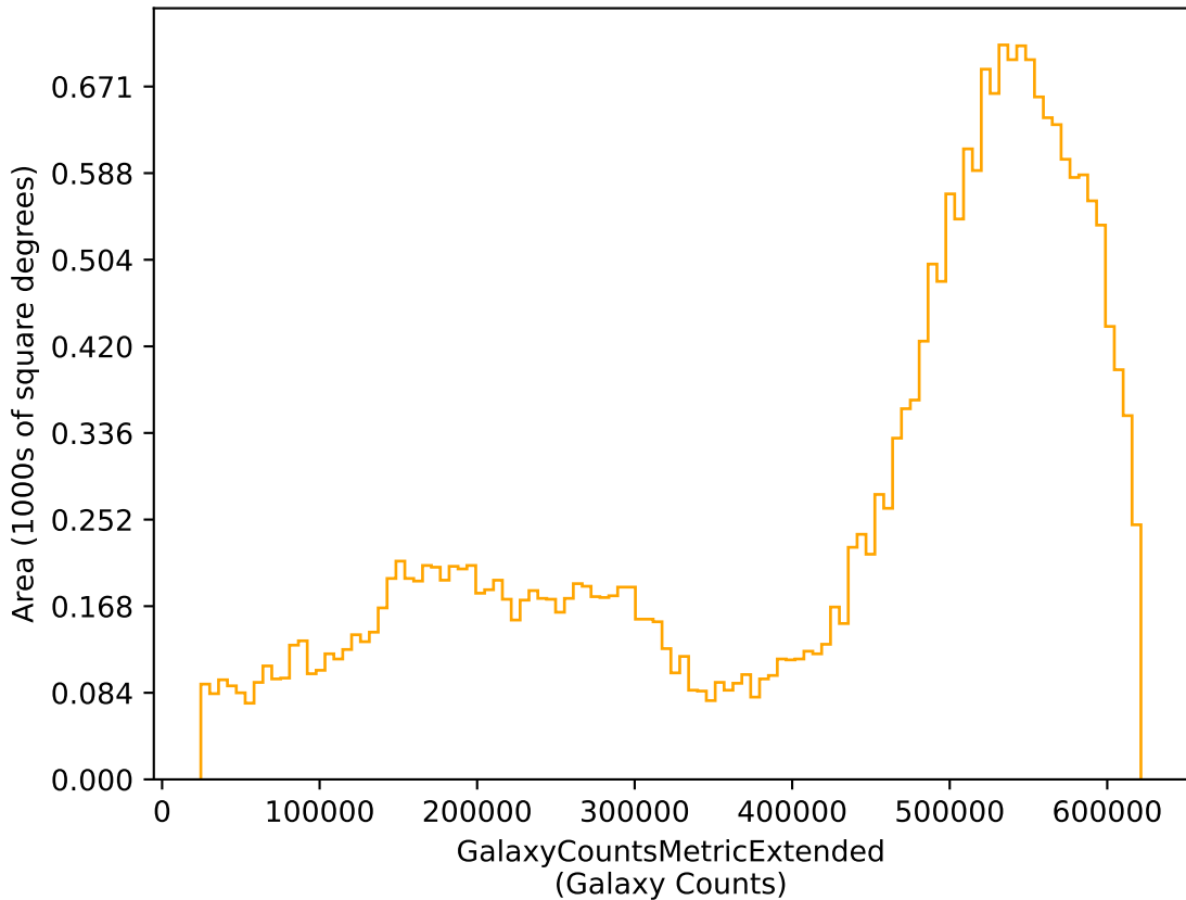
too_5_1v3.4_10yrs r: GalaxyCountsMetricExtended
