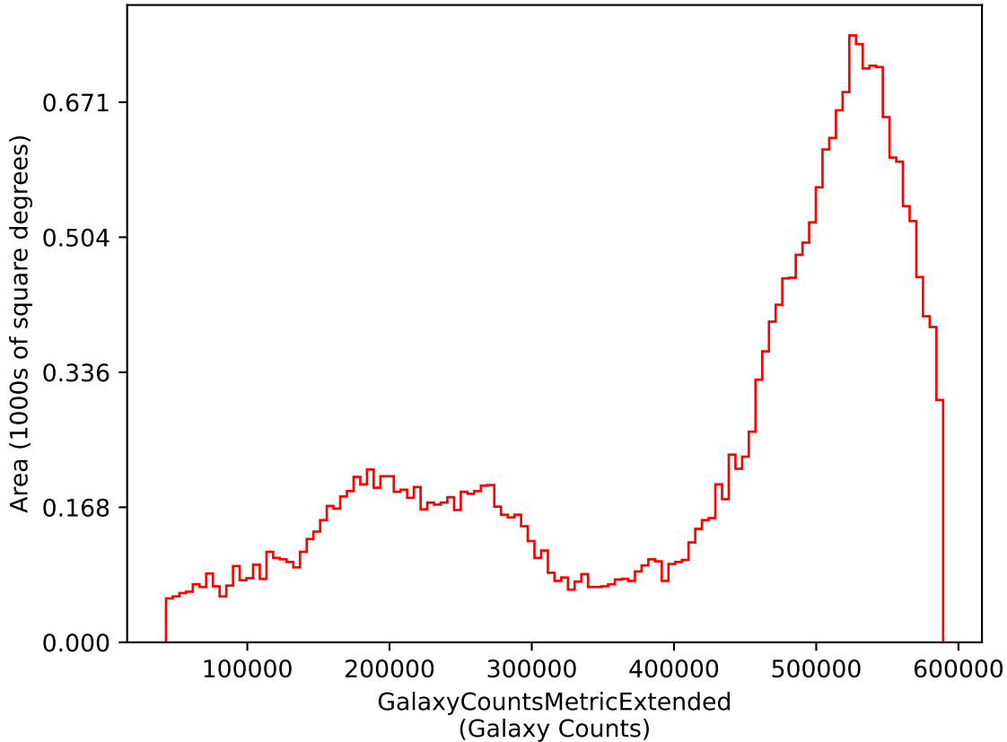
too_5_1v3.4_10yrs i: GalaxyCountsMetricExtended
