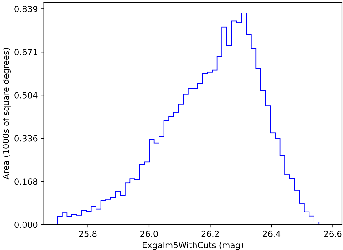
too_5_1v3.4_10yrs i band non-DD year 7: ExgalM5WithCuts
