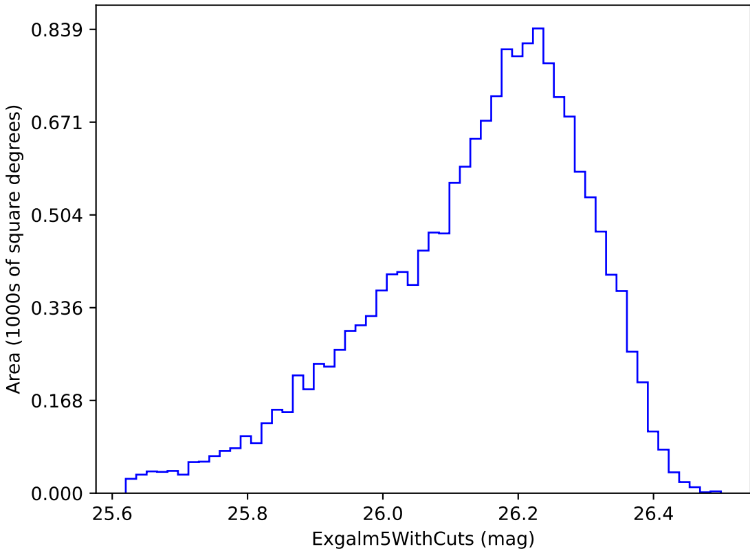
too_5_1v3.4_10yrs i band non-DD year 6: ExgalM5WithCuts
