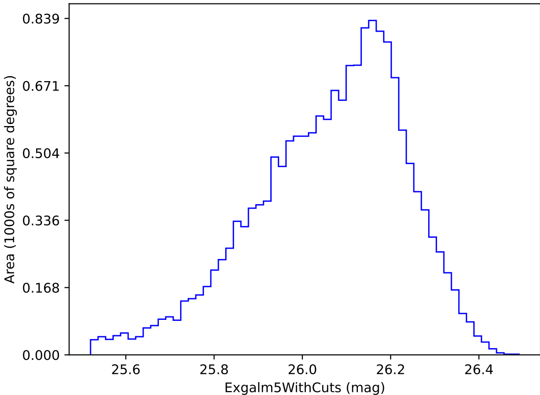
too_5_1v3.4_10yrs i band non-DD year 5: ExgalM5WithCuts
