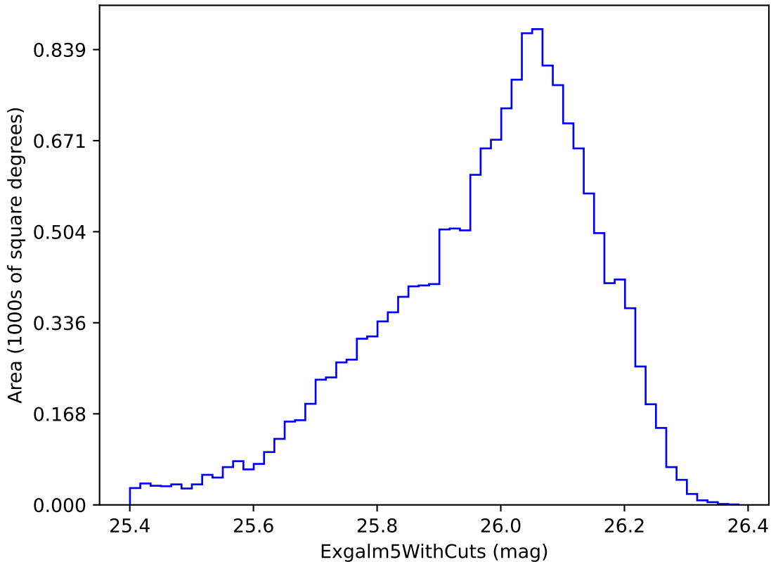
too_5_1v3.4_10yrs i band non-DD year 4: ExgalM5WithCuts
