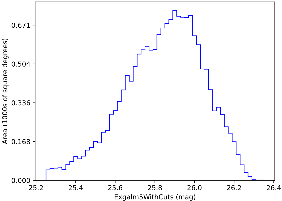
too_5_1v3.4_10yrs i band non-DD year 3: ExgalM5WithCuts
