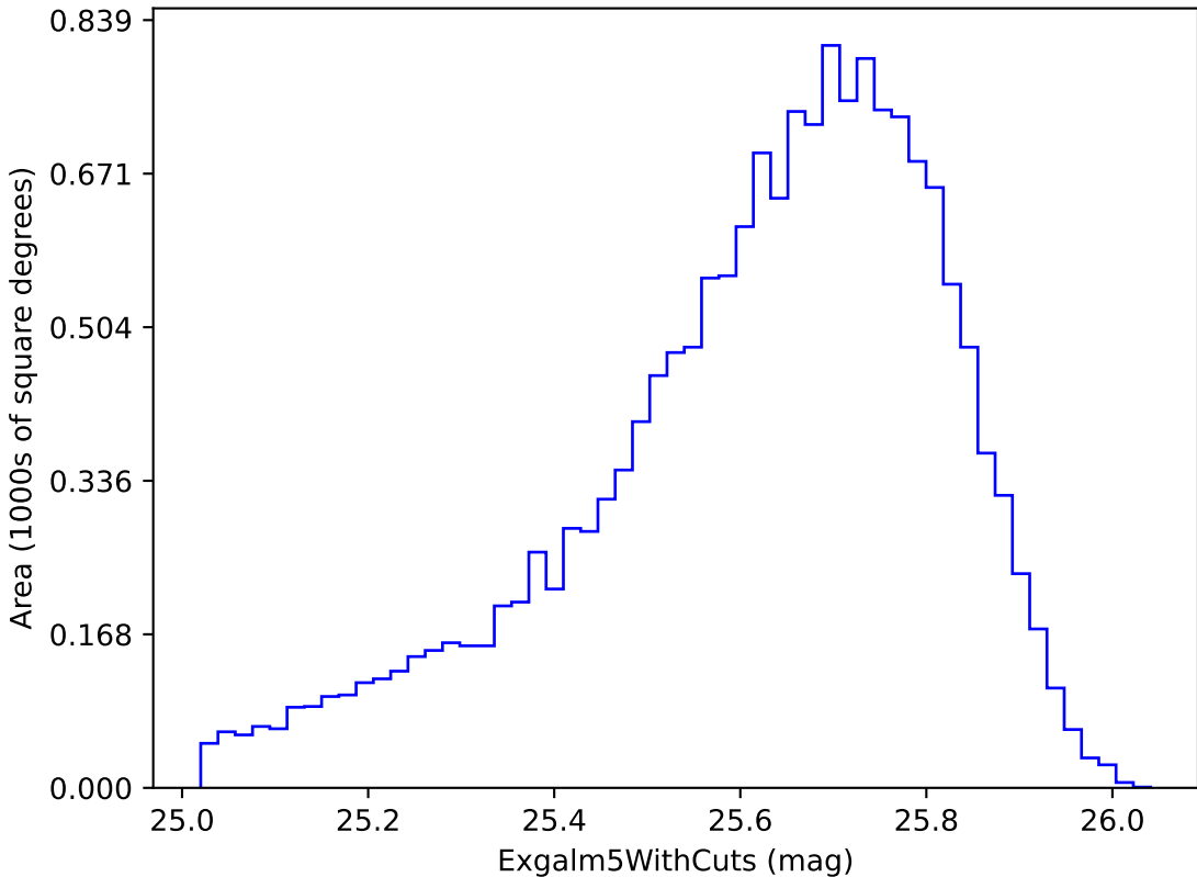
too_5_1v3.4_10yrs i band non-DD year 2: ExgalM5WithCuts
