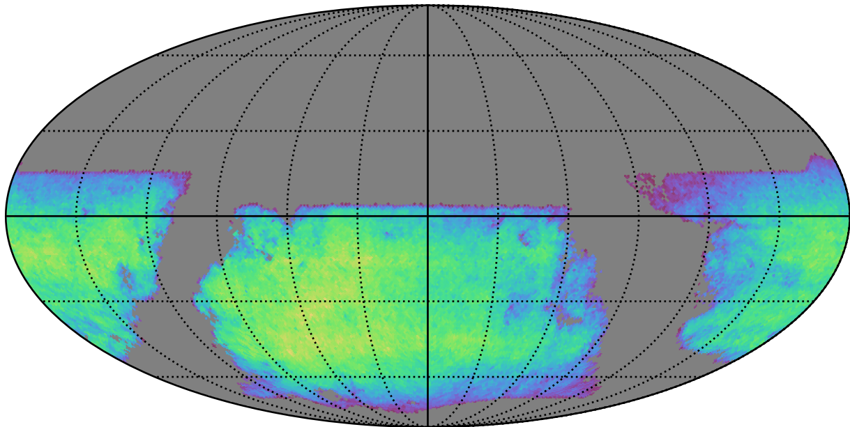
too_5_1v3.4_10yrs i band non-DD year 10: ExgalM5WithCuts
