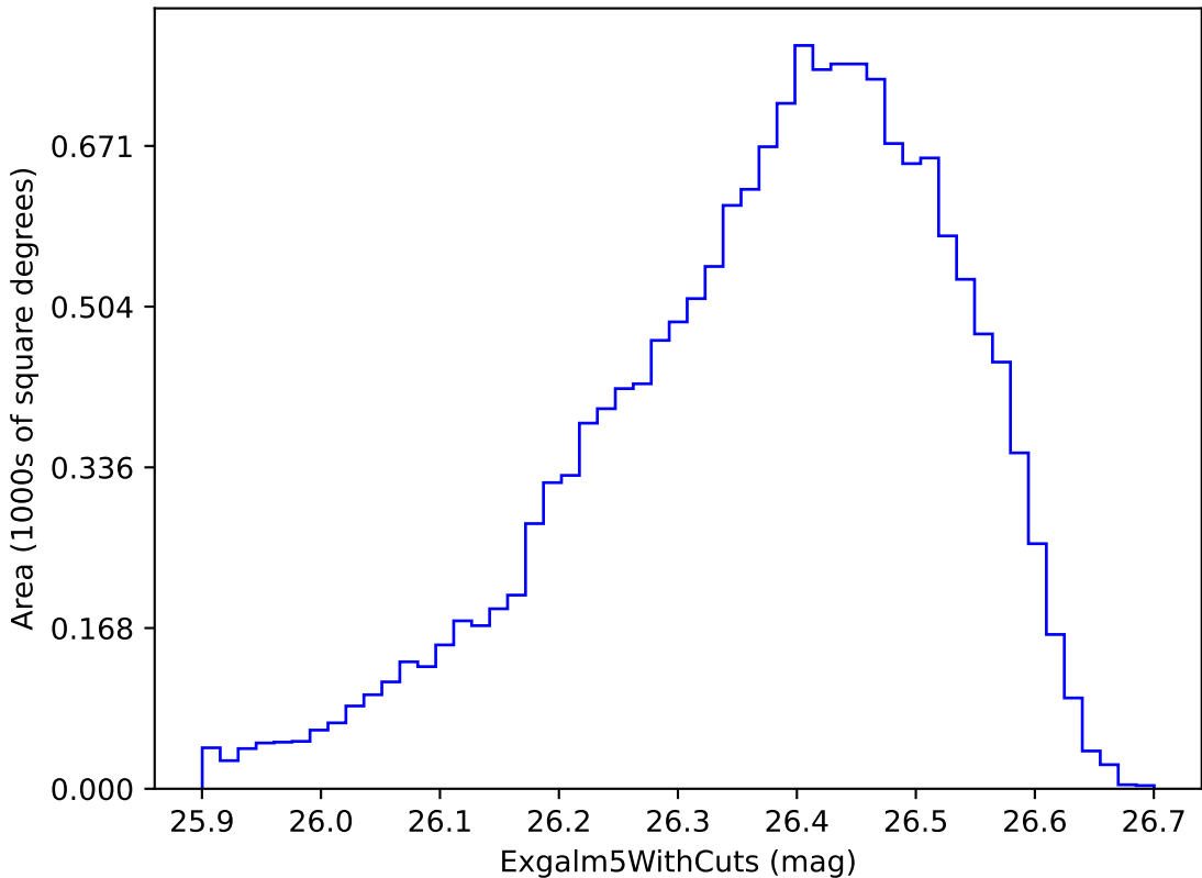
too_5_1v3.4_10yrs i band non-DD year 10: ExgalM5WithCuts
