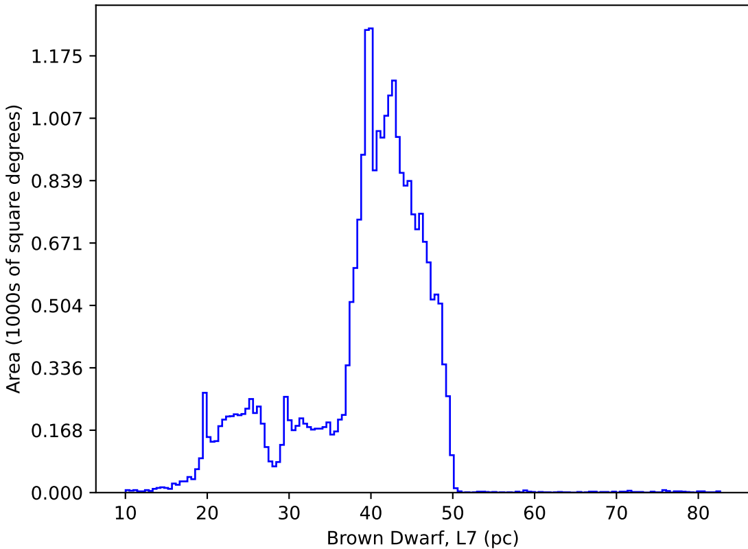
too_5_1v3.4_10yrs : Brown Dwarf, L7
