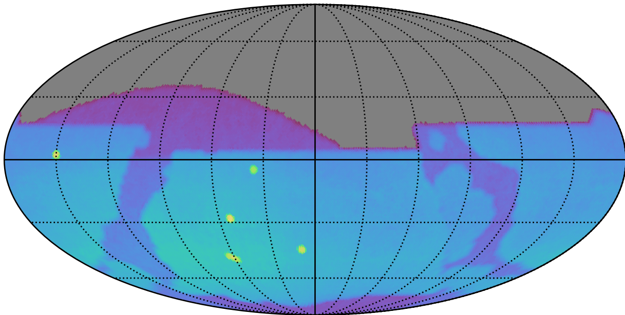
too_5_1v3.4_10yrs : Brown Dwarf, L4
