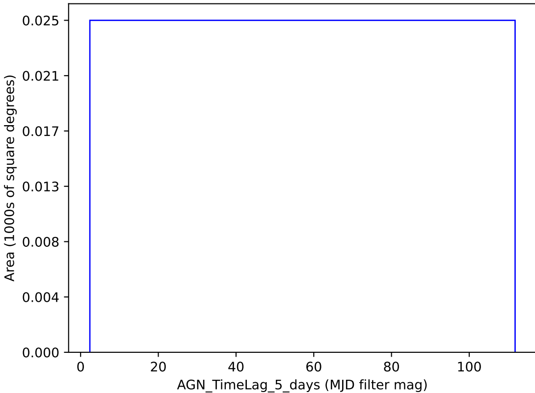
too_5_1v3.4_10yrs y band: AGN_TimeLag_5_days
