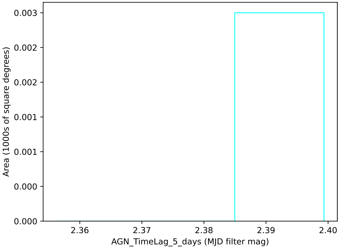
too_5_1v3.4_10yrs u band: AGN_TimeLag_5_days
