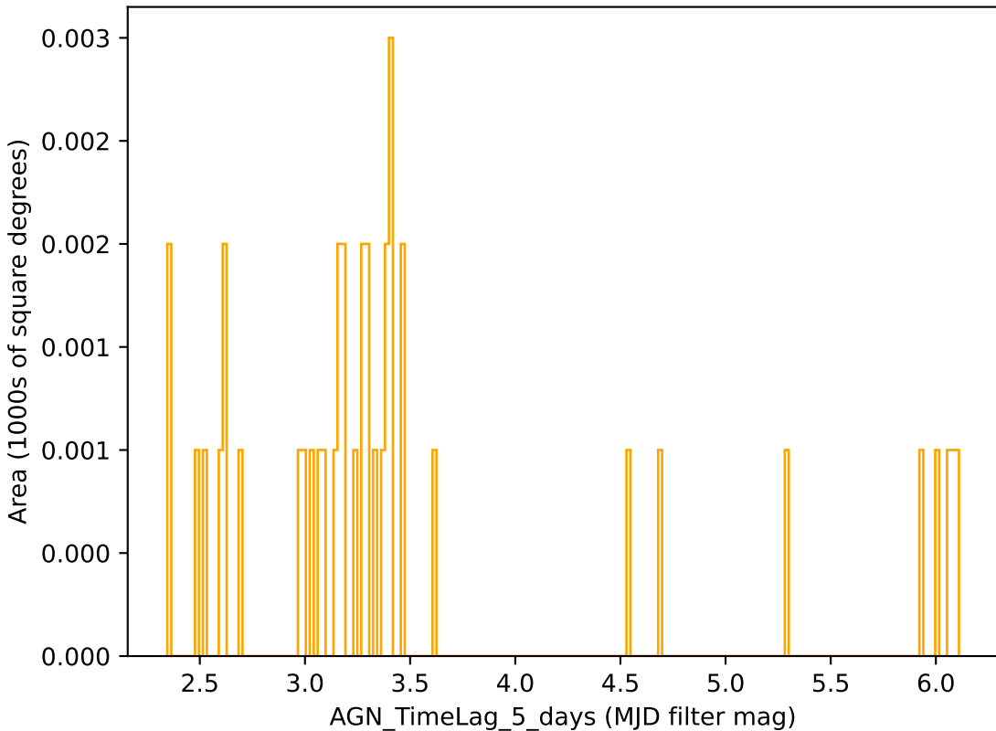
too_5_1v3.4_10yrs r band: AGN_TimeLag_5_days
