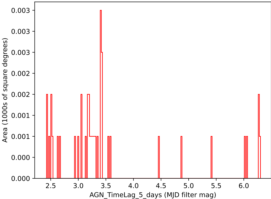
too_5_1v3.4_10yrs i band: AGN_TimeLag_5_days
