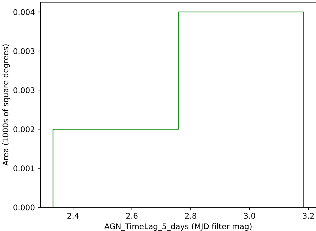
too_5_1v3.4_10yrs g band: AGN_TimeLag_5_days
