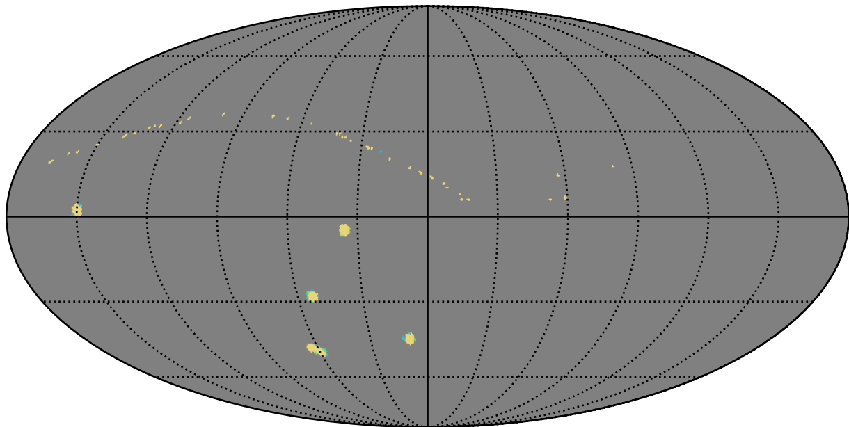
too_5_1v3.4_10yrs all bands: AGN_TimeLag_5_days
