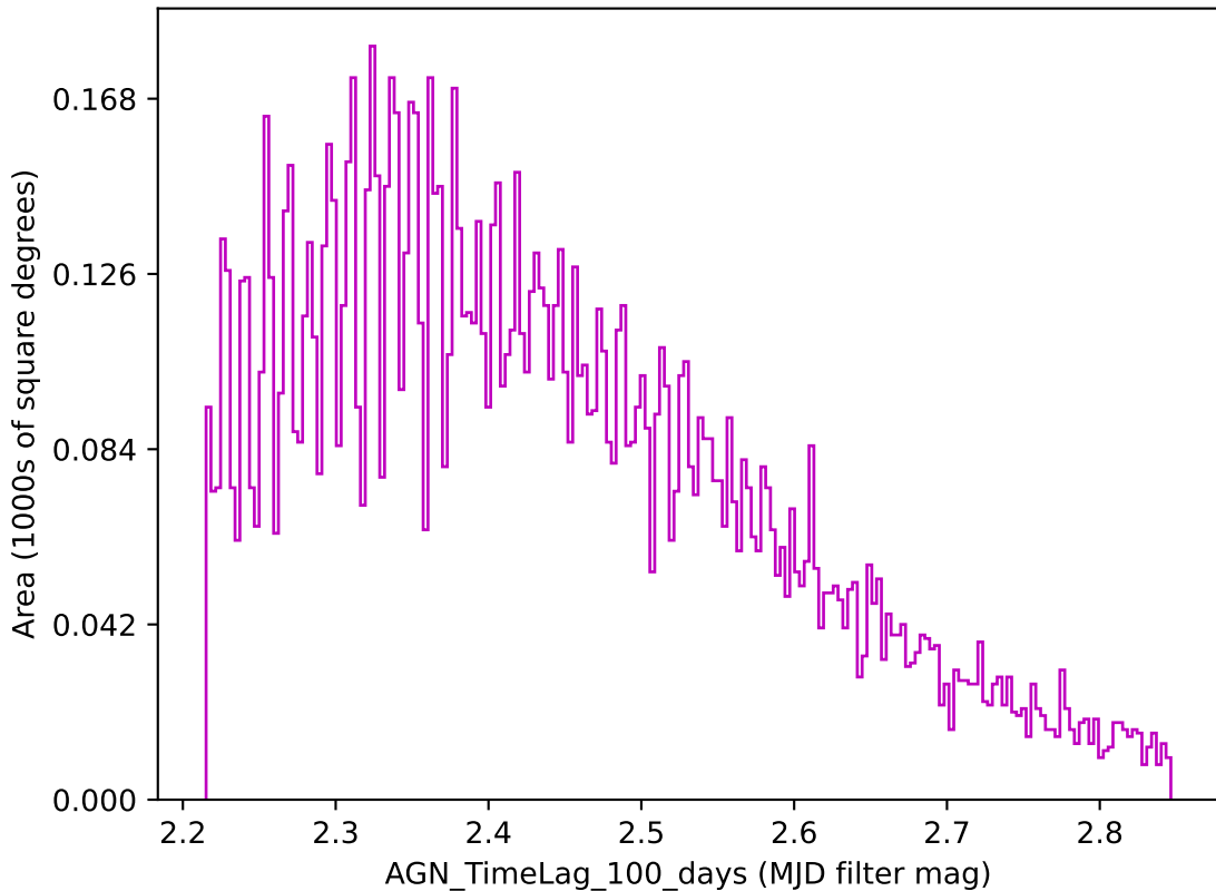
too_5_1v3.4_10yrs z band: AGN_TimeLag_100_days
