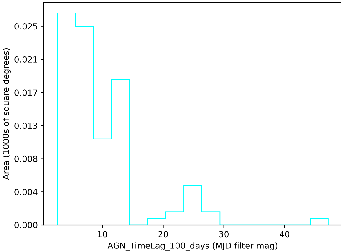
too_5_1v3.4_10yrs u band: AGN_TimeLag_100_days
