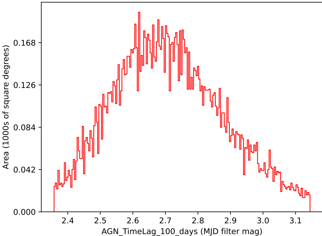
too_5_1v3.4_10yrs i band: AGN_TimeLag_100_days
