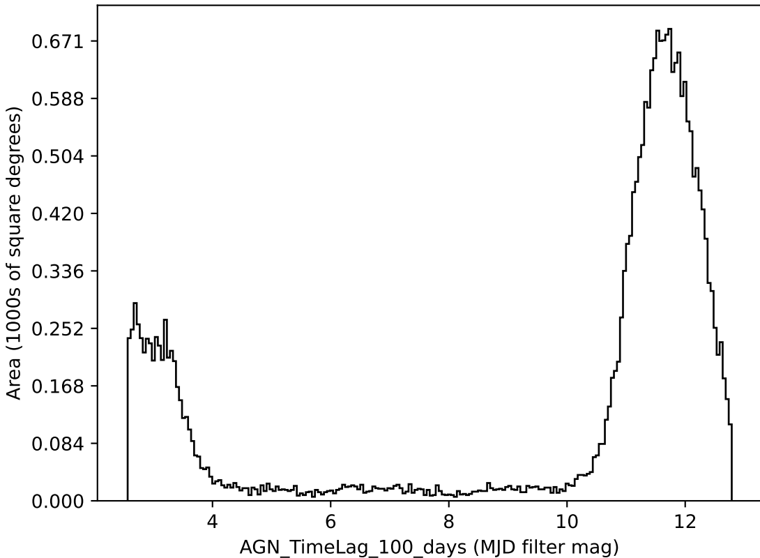
too_5_1v3.4_10yrs all bands: AGN_TimeLag_100_days
