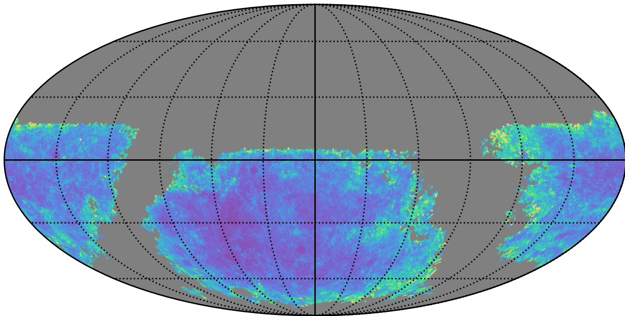
too_5_1v3.4_10yrs u band: AGN SF_uncert
