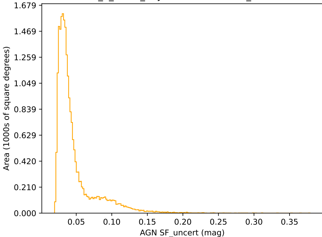
too_5_1v3.4_10yrs r band: AGN SF_uncert
