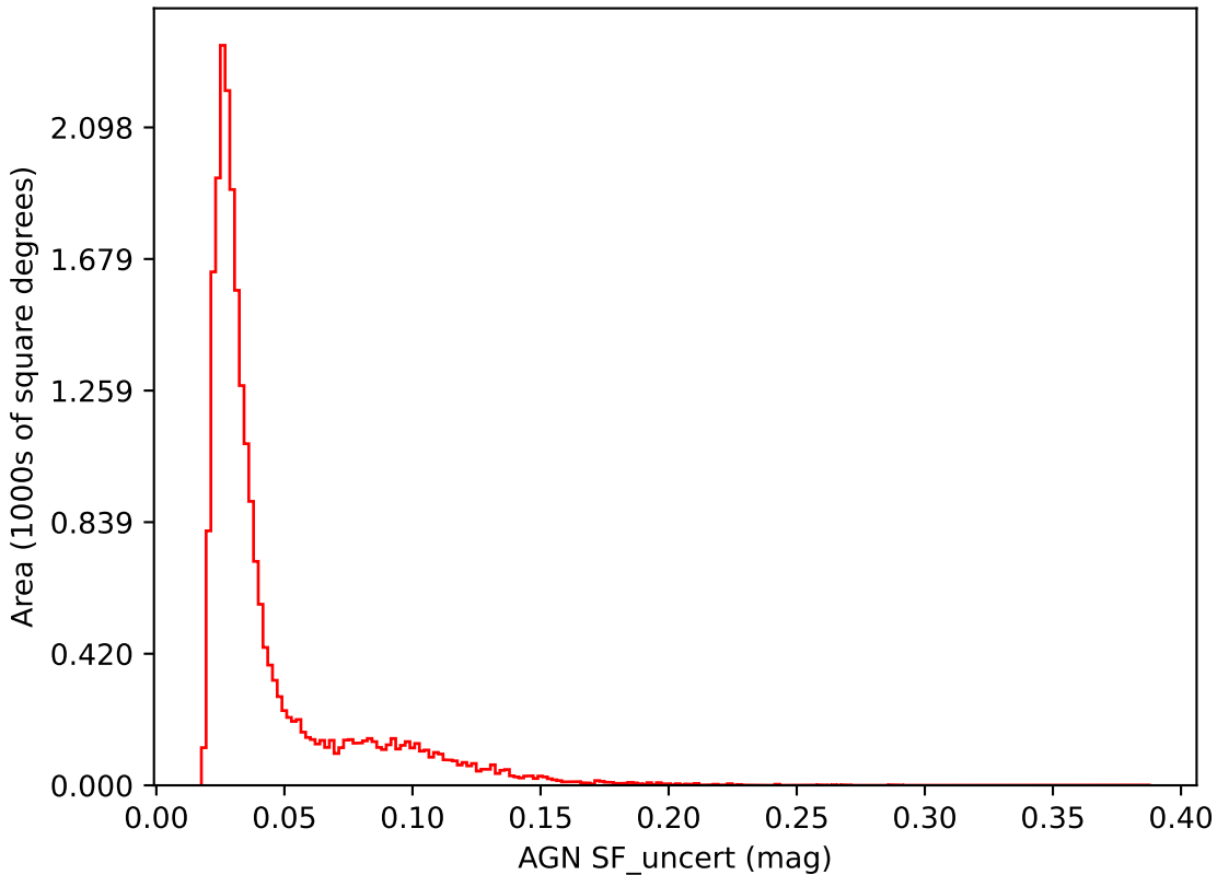
too_5_1v3.4_10yrs i band: AGN SF_uncert
