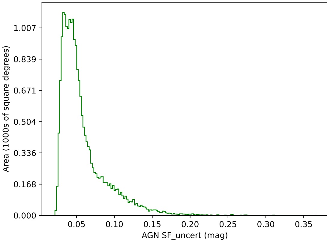
too_5_1v3.4_10yrs g band: AGN SF_uncert
