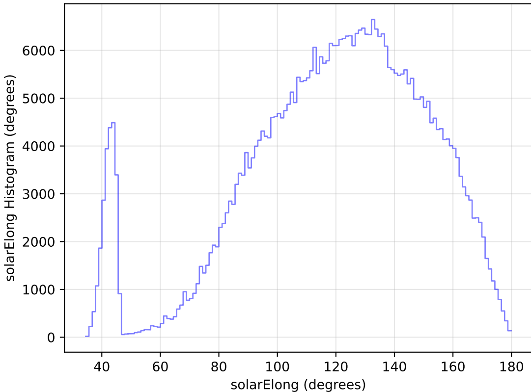
too_5_1v3.4_10yrs WFD z band: solarElong Histogram
