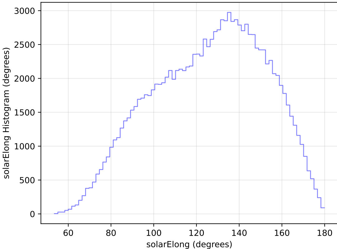
too_5_1v3.4_10yrs WFD u band: solarElong Histogram
